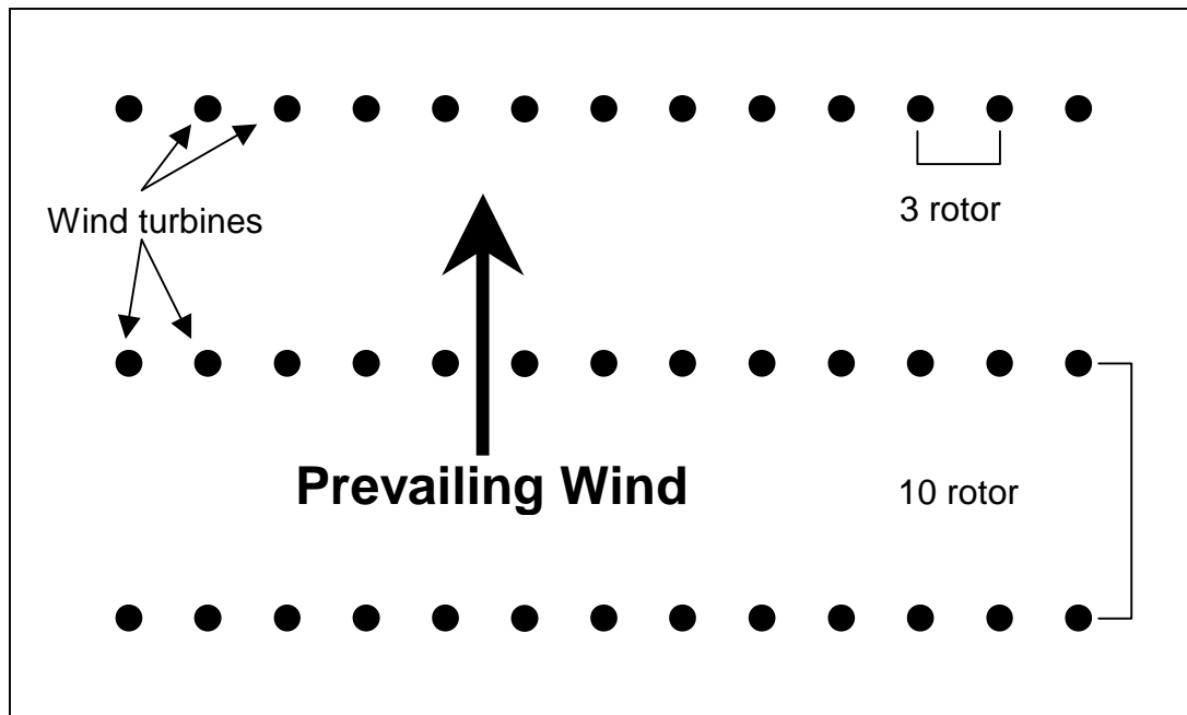
Figure 2. Illustration of Turbine Spacing (example: 3 x 10 spacing)
