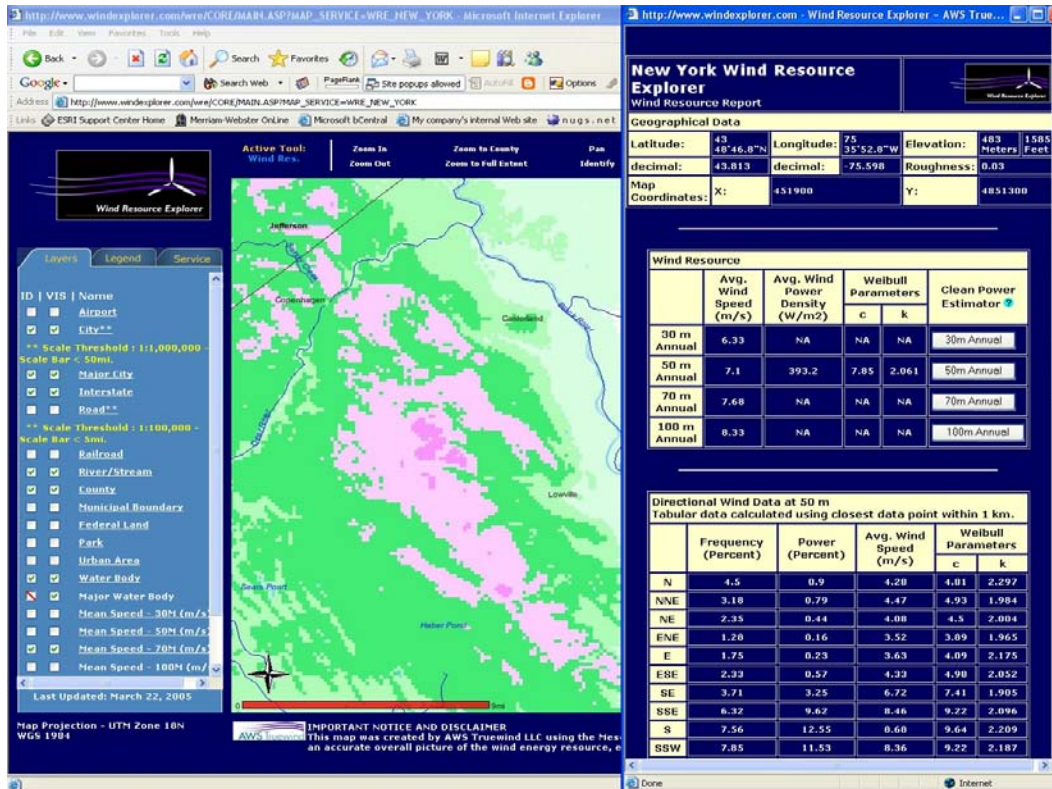
Figure 1. Example of Wind Map For A Portion of the Tug Hill Plateau Region of New York
